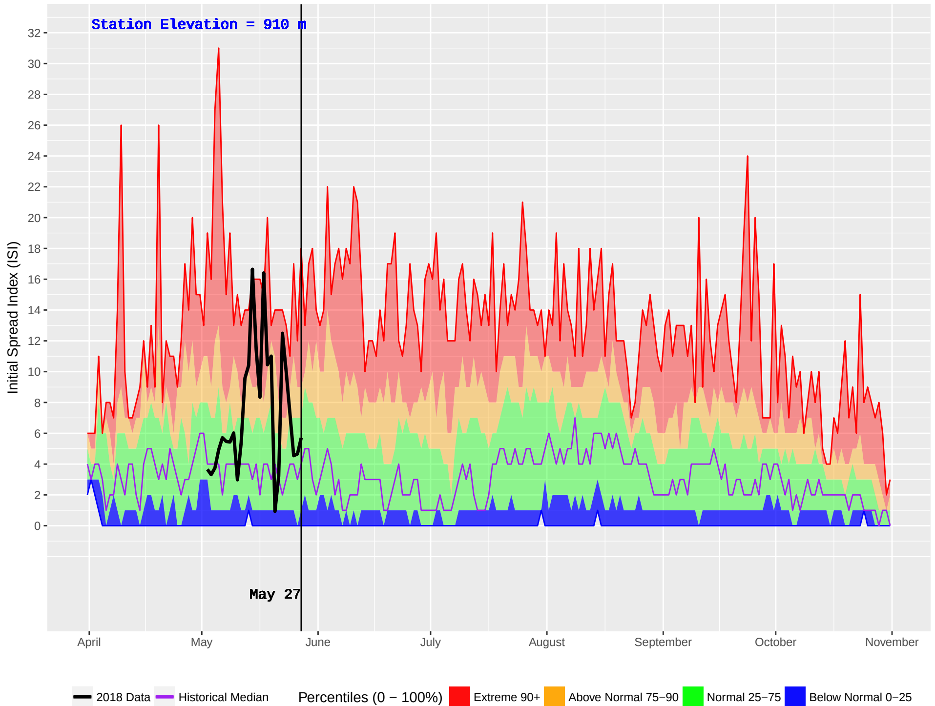
NAZKO (211) : Historical (1981–2016) and Current (2018) Noon Initial Spread Index (ISI)
