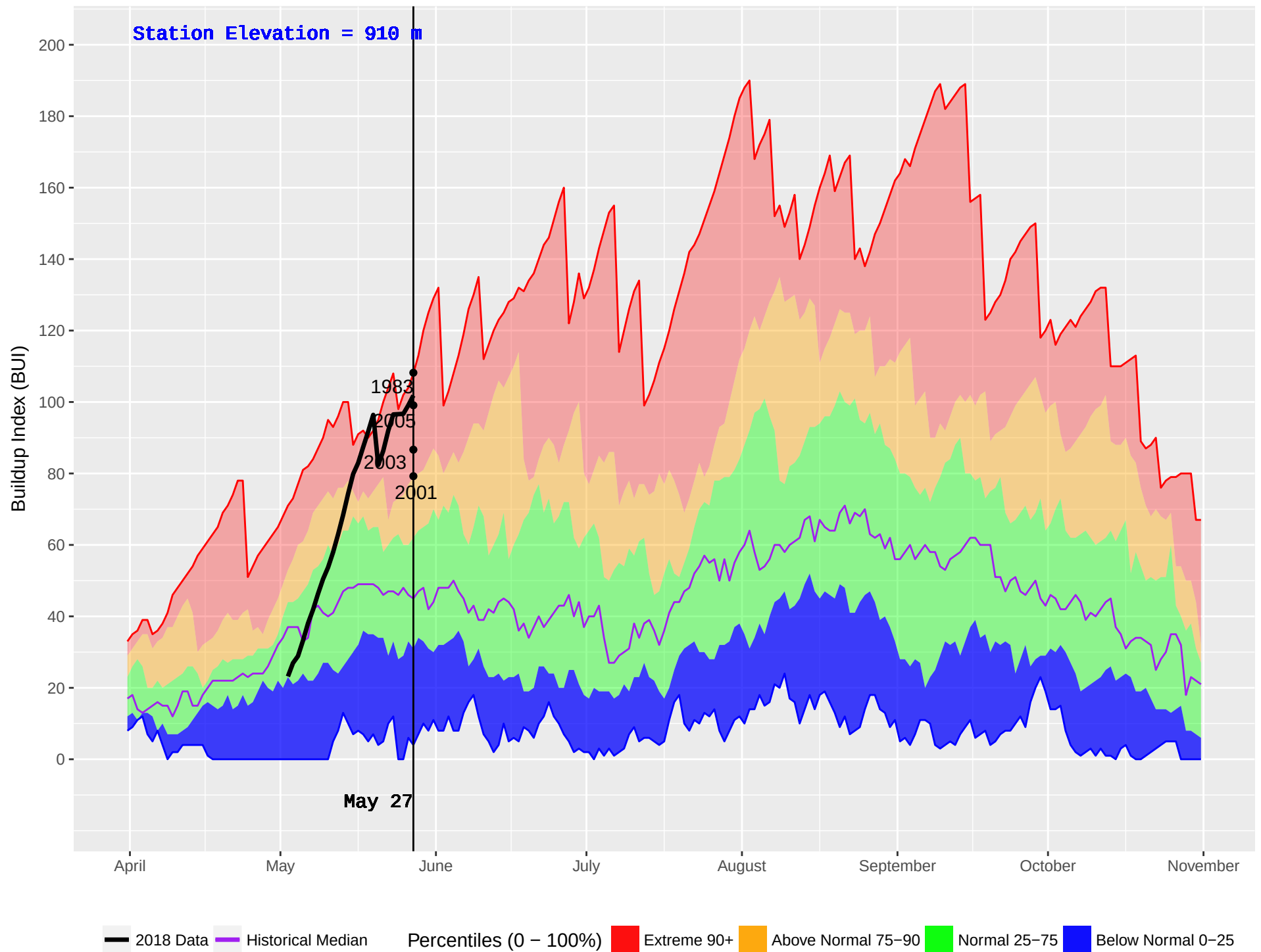
NAZKO (211) : Historical (1981–2016) and Current (2018) Noon Buildup Index (BUI)
