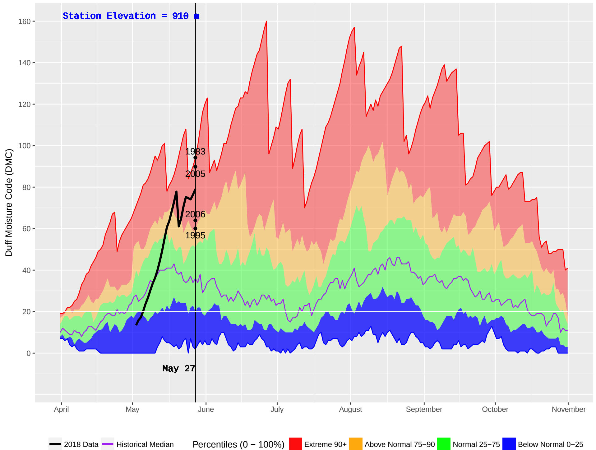
NAZKO (211) : Historical (1981–2016) and Current (2018) Noon Duff Moisture Code (DMC)
