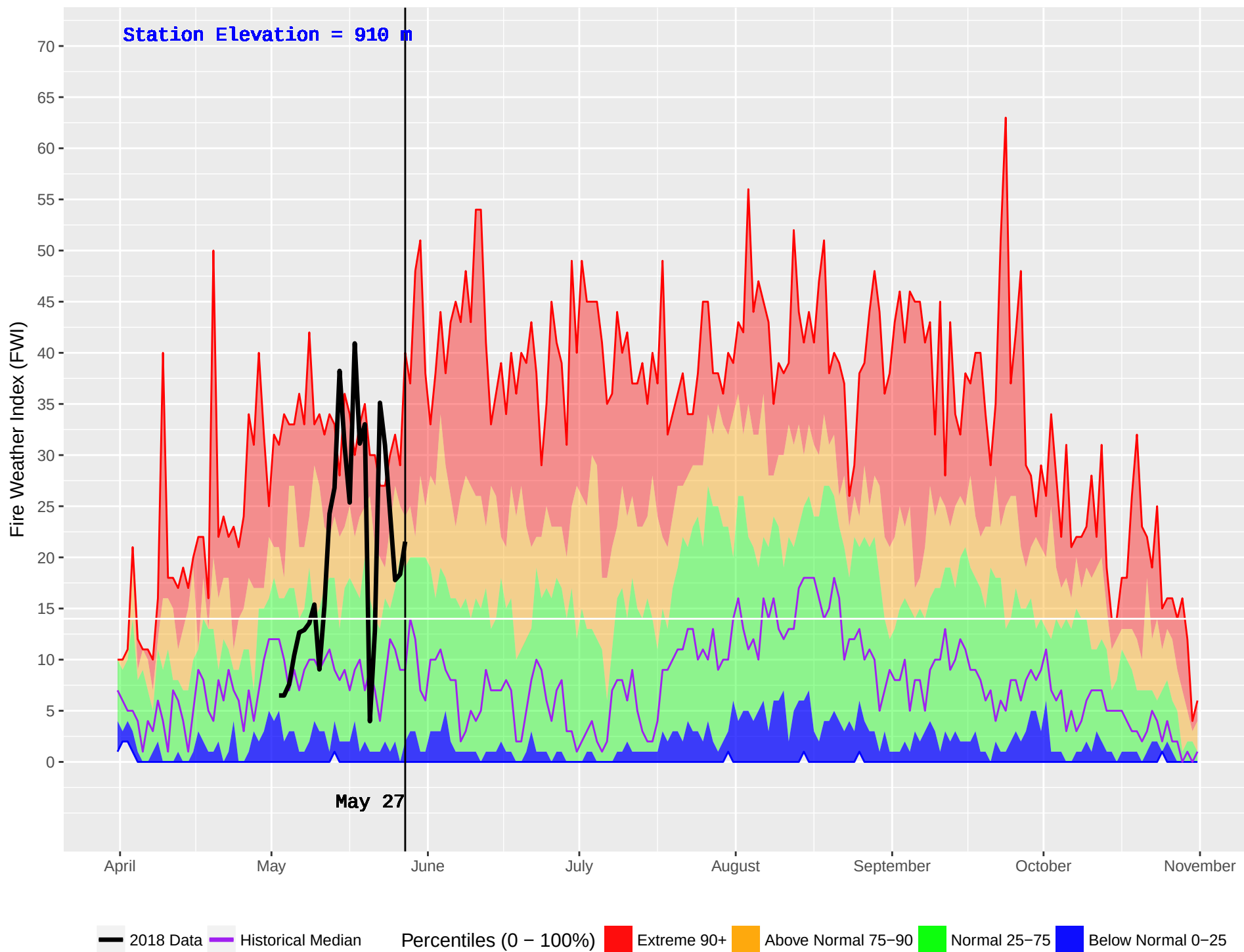
NAZKO (211) : Historical (1981–2016) and Current (2018) Noon Fire Weather Index (FWI)
