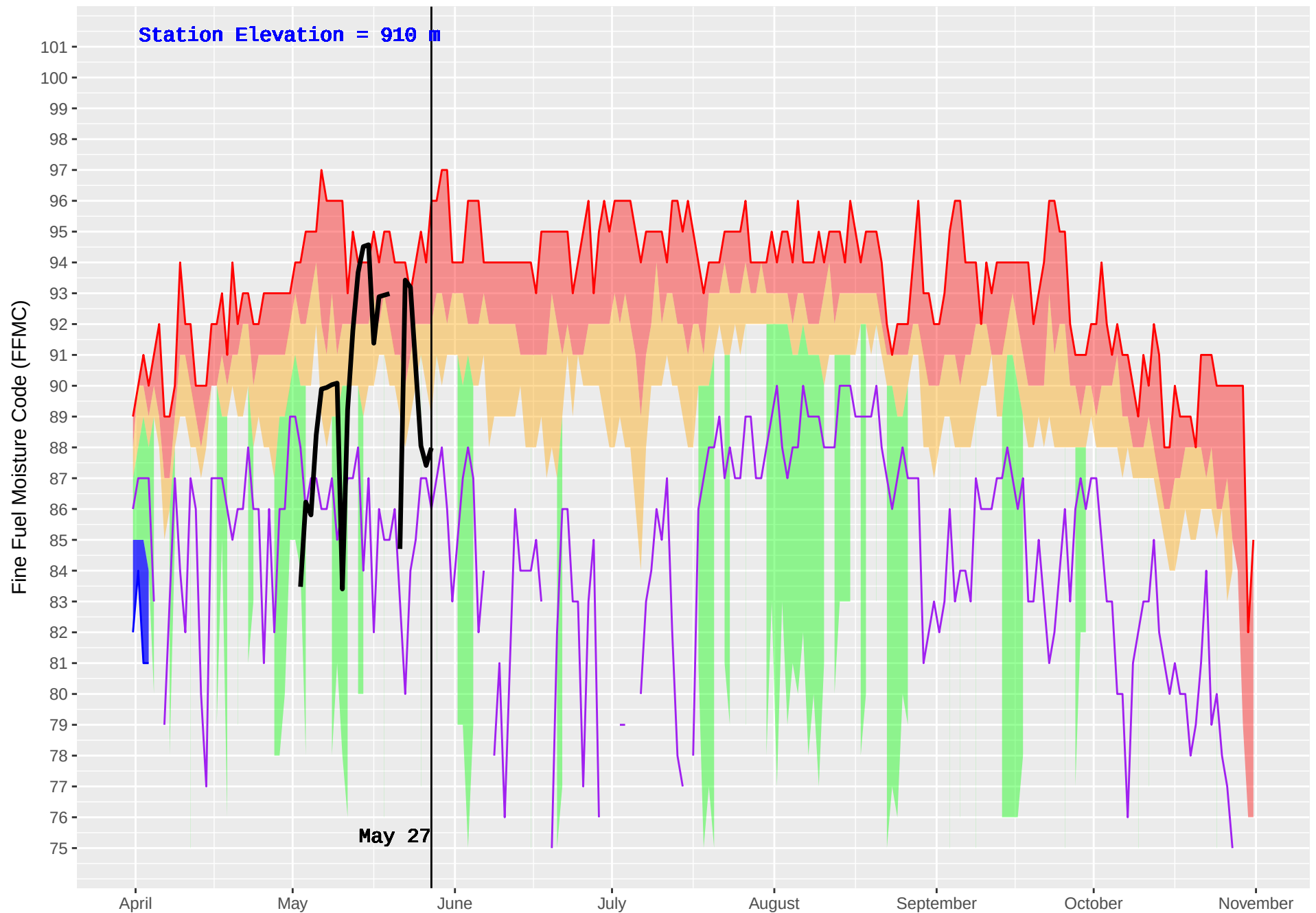
NAZKO (211) : Historical (1981–2016) and Current (2018) Noon Fine Fuel Moisture Code (FFMC)
